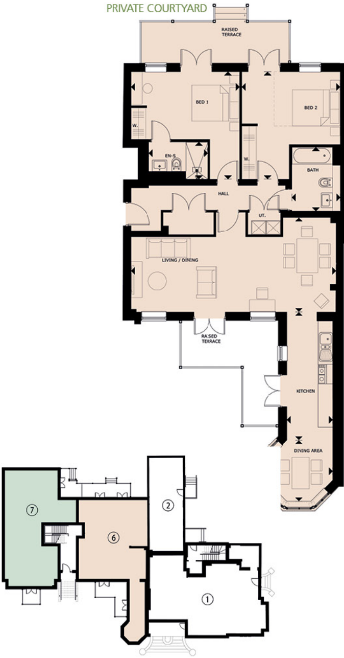
Plot 6 - Ground Floor Plan
