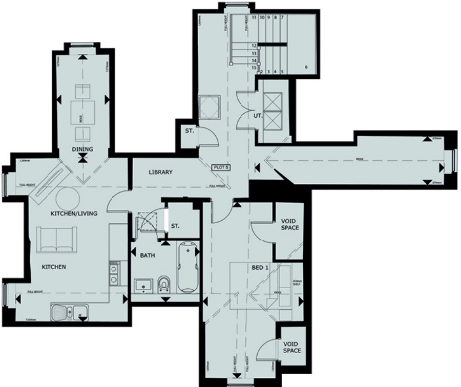
FIRST FLOOR
